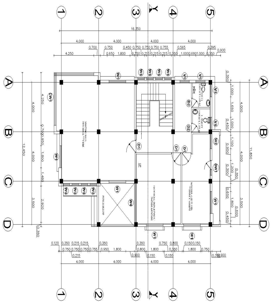
WARD BUILDING FIRST FLOOR PLAN AREA- 165.7475 SQ. M.
