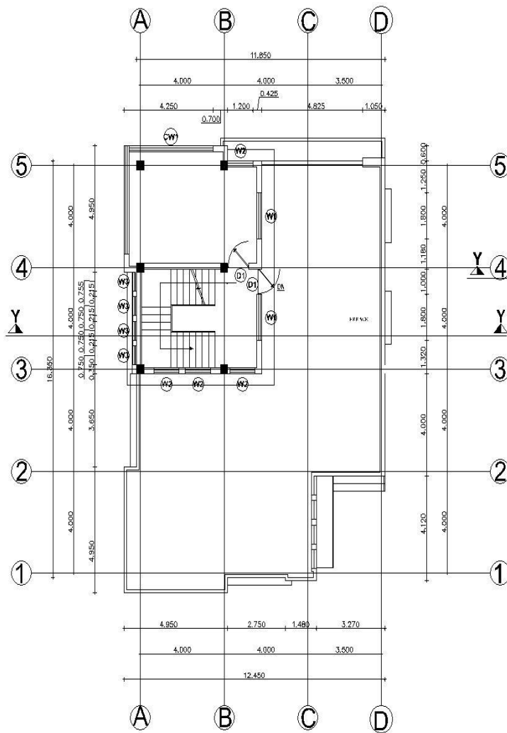
WARD BUILDING SECOND FLOOR PLAN AREA- 165.7475 SQ. M.
